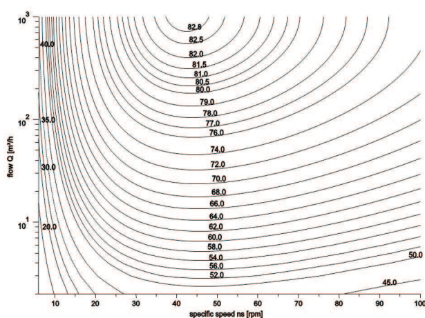
MEI=0.7 for Mutistage Vertical 2900 rpm
